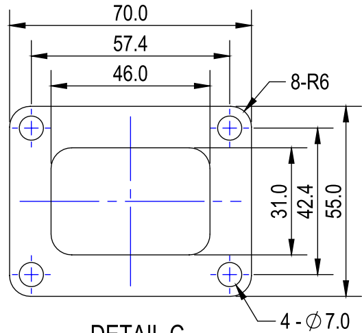
DETAIL C SCALE 2 : 3
